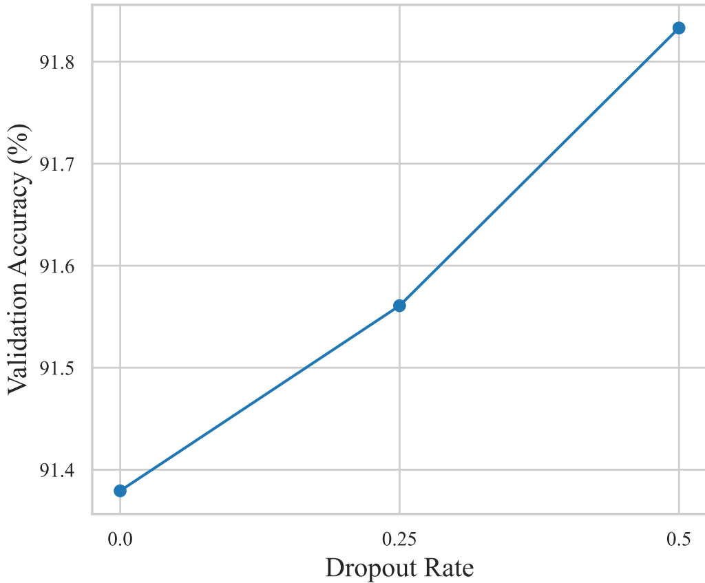
Plot 10: Dropout Rate vs. Validation Accuracy
